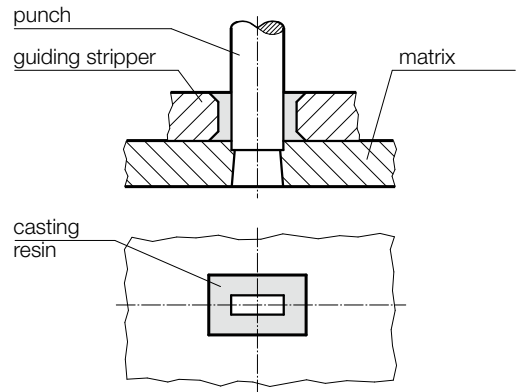
Fig. 3: Casting of punch guide with basic blanking tools
