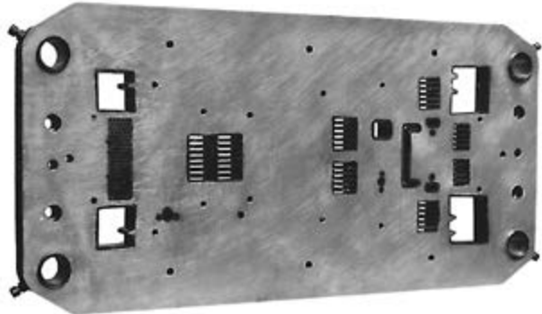
Fig. 7 Cast punch guide plate
