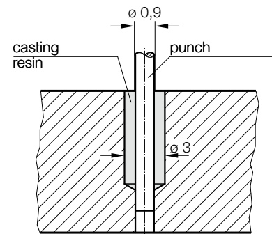
Fig. 5: Cast guide for thin Quill-Type Punch
