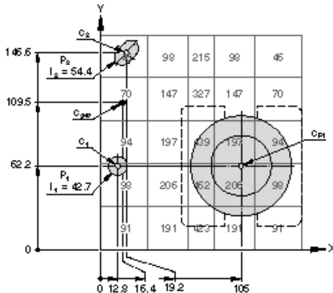
Figure 24: Eccentric hole pattern with compensation spring
